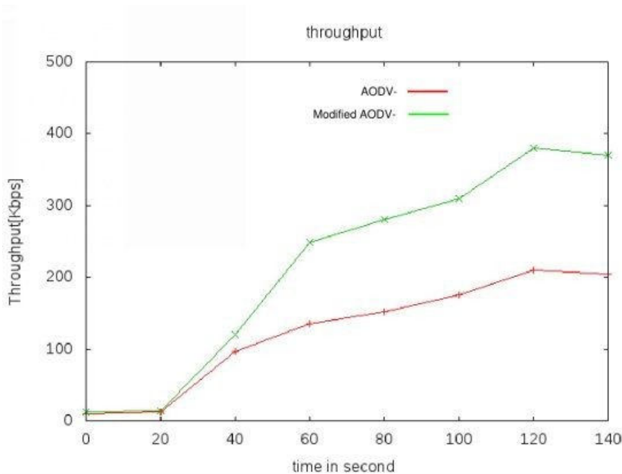
Fig 2: Throughput
